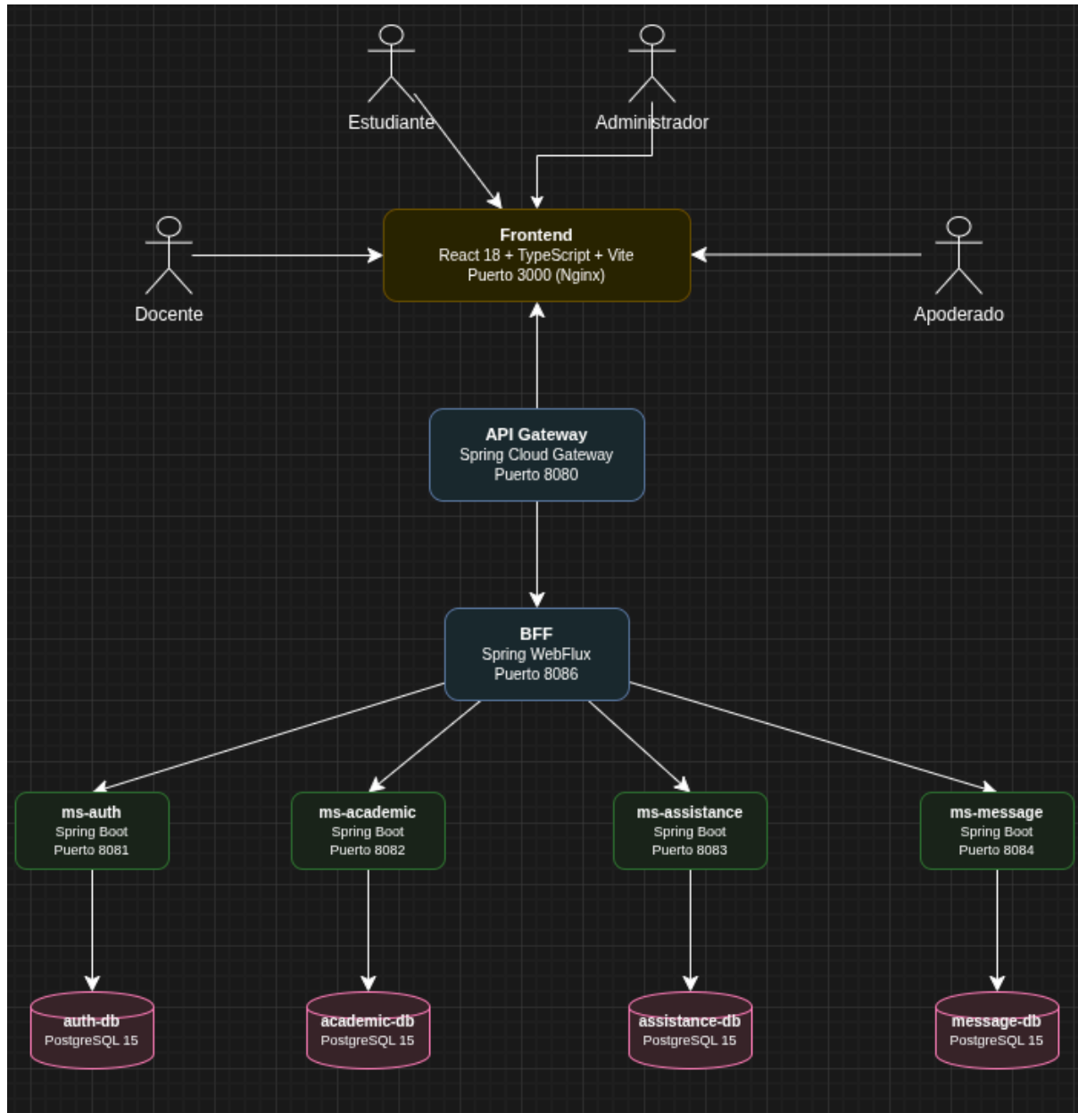
Fig 2. Diagrama C2
