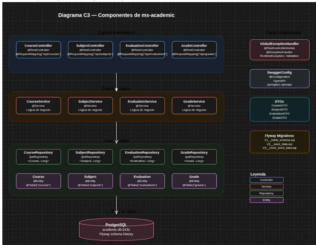
Fig 3. Diagrama C3
